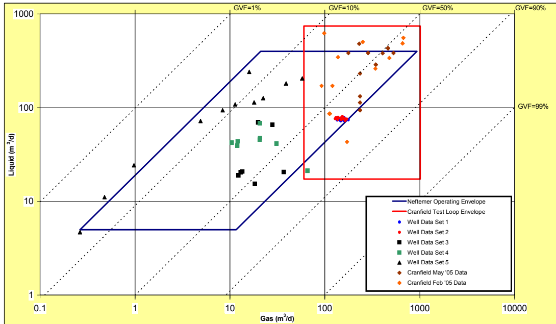
Figure 4 – Neftemer Operating Envelope
