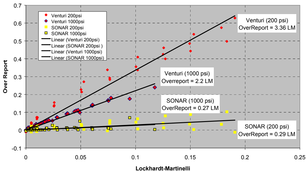
Figure 3: Over Reading of SONAR and Venturi Meters as a Function of Lockhardt-Martinelli Number
